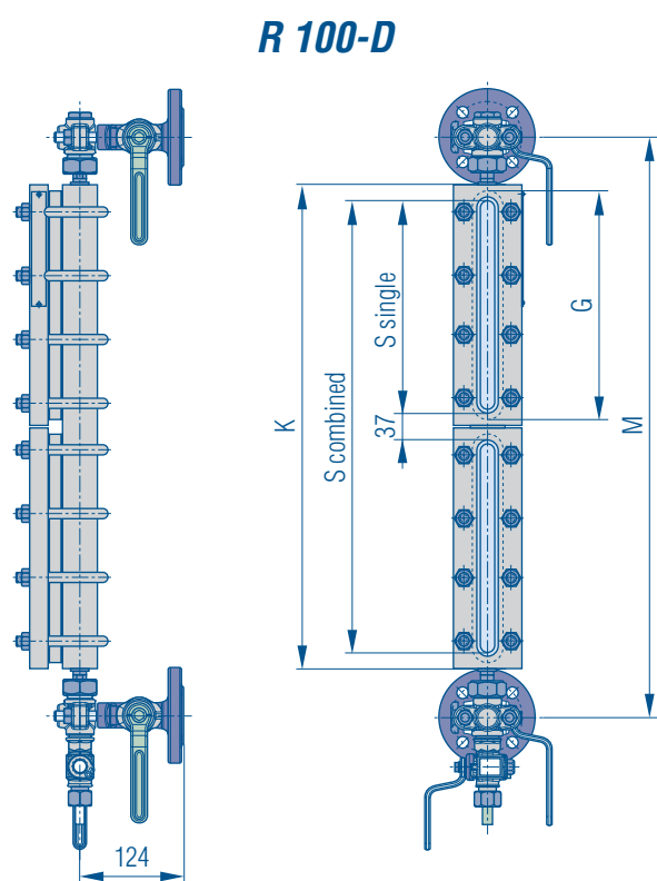
Overall and connection dimensions (mm)
