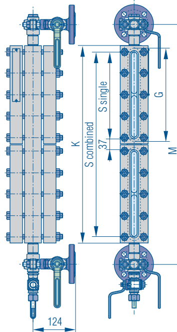
Overall and connection dimensions (mm)
